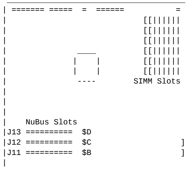
PowerMacintosh 8100 / Workgroup Server 8150 Board Layout
