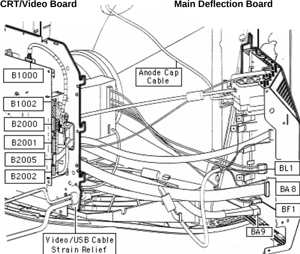
CRT/Video Board
